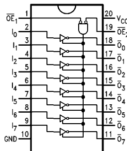
Figure 2. Connection Diagram
