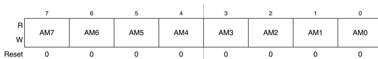
Figure 18-23. MSCAN Identifier Mask Registers (Second Bank) — CANIDMR4–CANIDMR7
