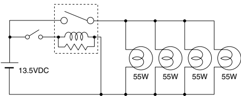
Circuit
