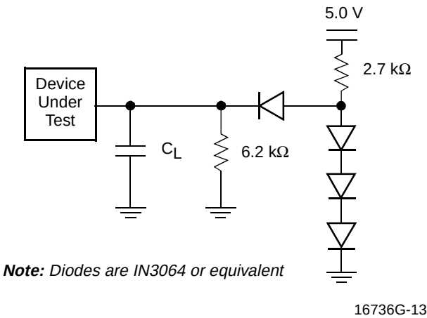
Figure 7. Test Setup
