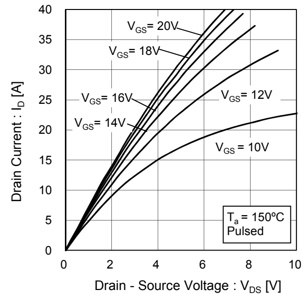
Fig.6 Typical Output Characteristics(I)
