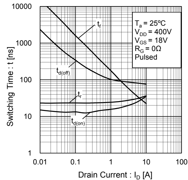
Fig.17 Switching Characteristics
