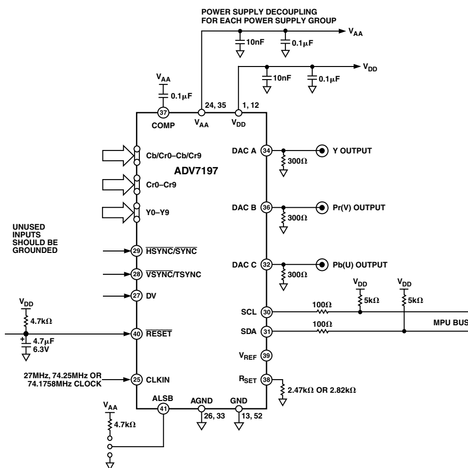
Figure 24. Circuit Layout
