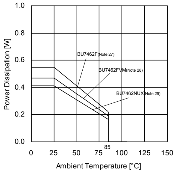
(e) BU7462xxx
