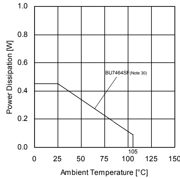
(h) BU7464SF
