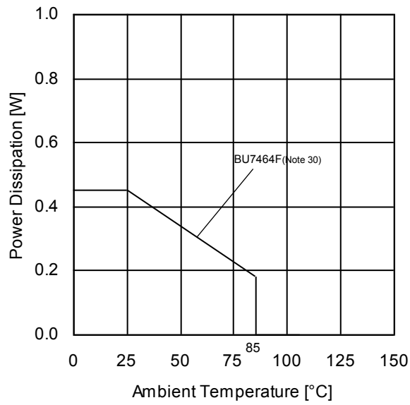
(g) BU7464F
