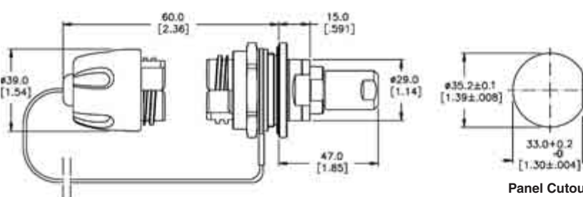
PRO BEAM Sr. D-Hole Bulkhead with Standard Cable Adapter
