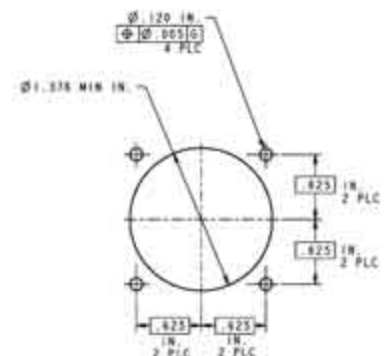
RECOMMENDED TFOCA-II ® PANEL CUT-OUT (DIMENSIONS: INCHES)
