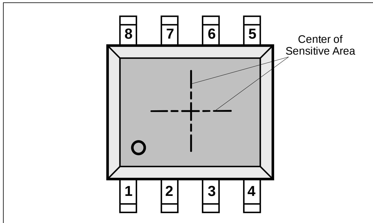
Figure 1 Pin Configuration
