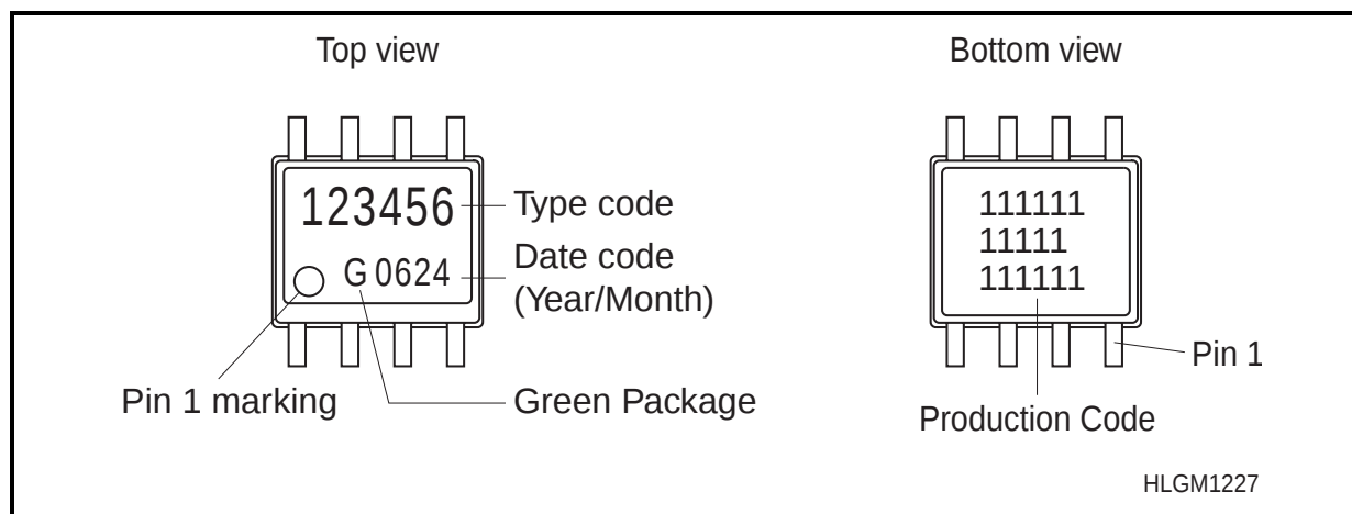
Figure 24 Marking
