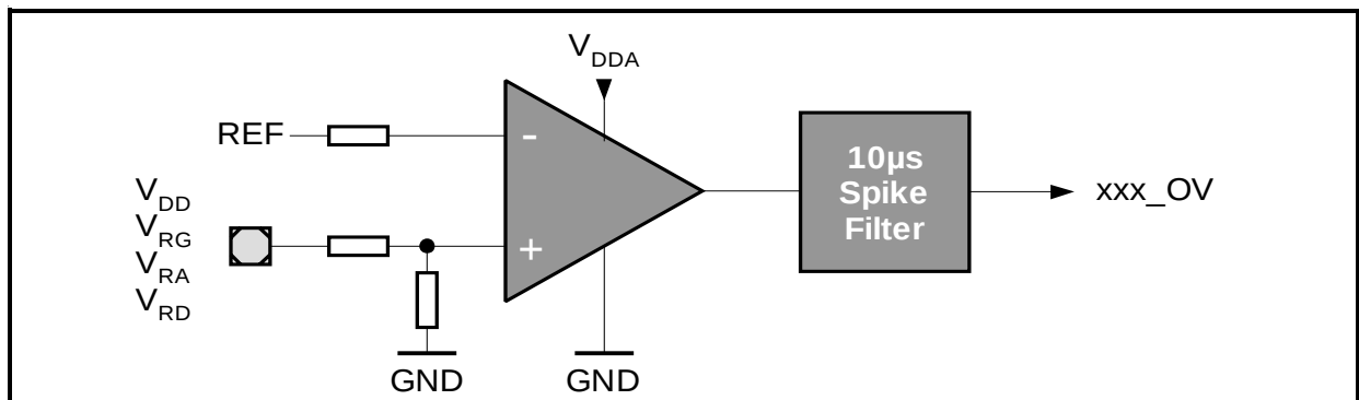
Figure 17 OV Comparator
