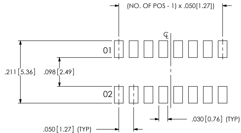
FIG 4 SURFACE MOUNT PASS THRU ENTRY (-108 POSITION SHOWN) ALL DIMENSION ARE SYMMETRICAL ABOUT THE CENTERLINE
