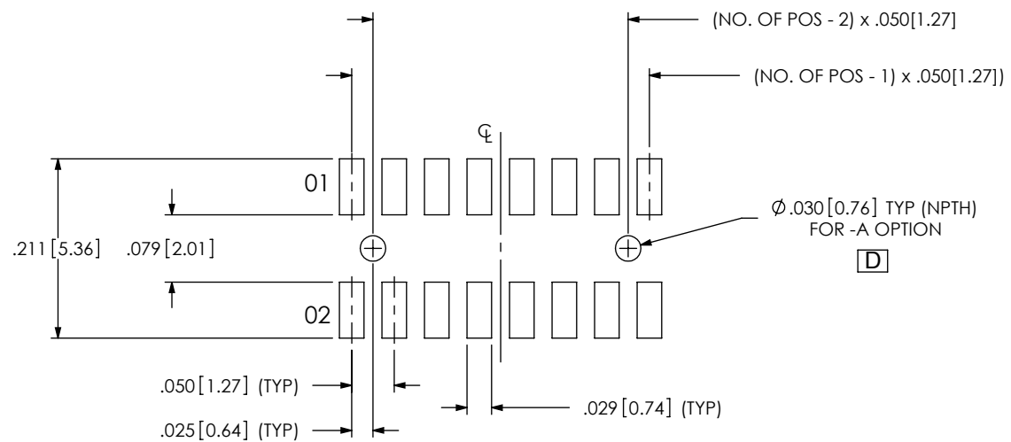
FIG 1 SURFACE MOUNT NON-PASS THRU ENTRY (-108 POSITION SHOWN) ALL DIMENSION ARE SYMMETRICAL ABOUT THE CENTERLINE
