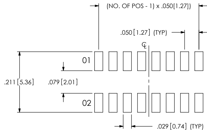
FIG 3 SURFACE MOUNT NON-PASS THRU ENTRY (-108 POSITION SHOWN) ALL DIMENSION ARE SYMMETRICAL ABOUT THE CENTERLINE
