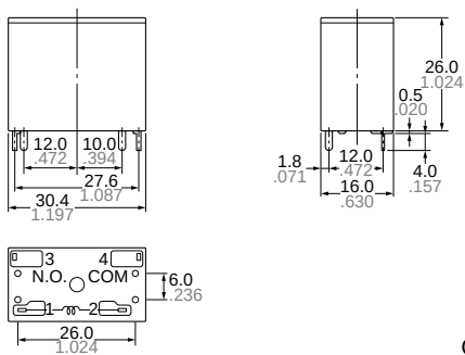
External dimensions
