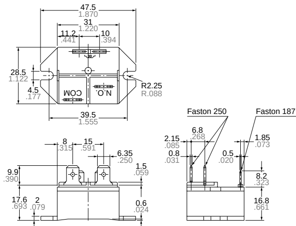
External dimensions
