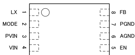
Figure 2. Pin Configuration(s)
