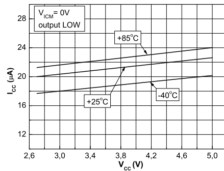
Figure 3. Supply current versus supply voltage with output low
