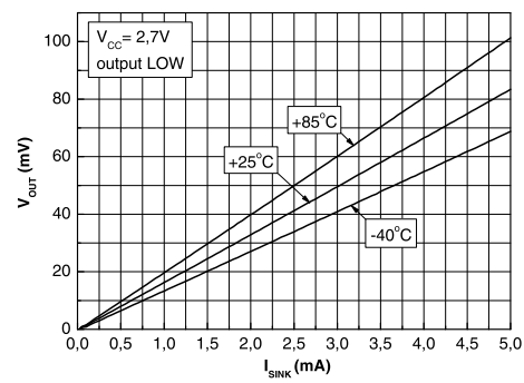
Figure 5. Output voltage versus output current at 2.7 V supply
