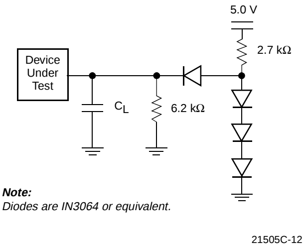
Figure 8. Test Setup
