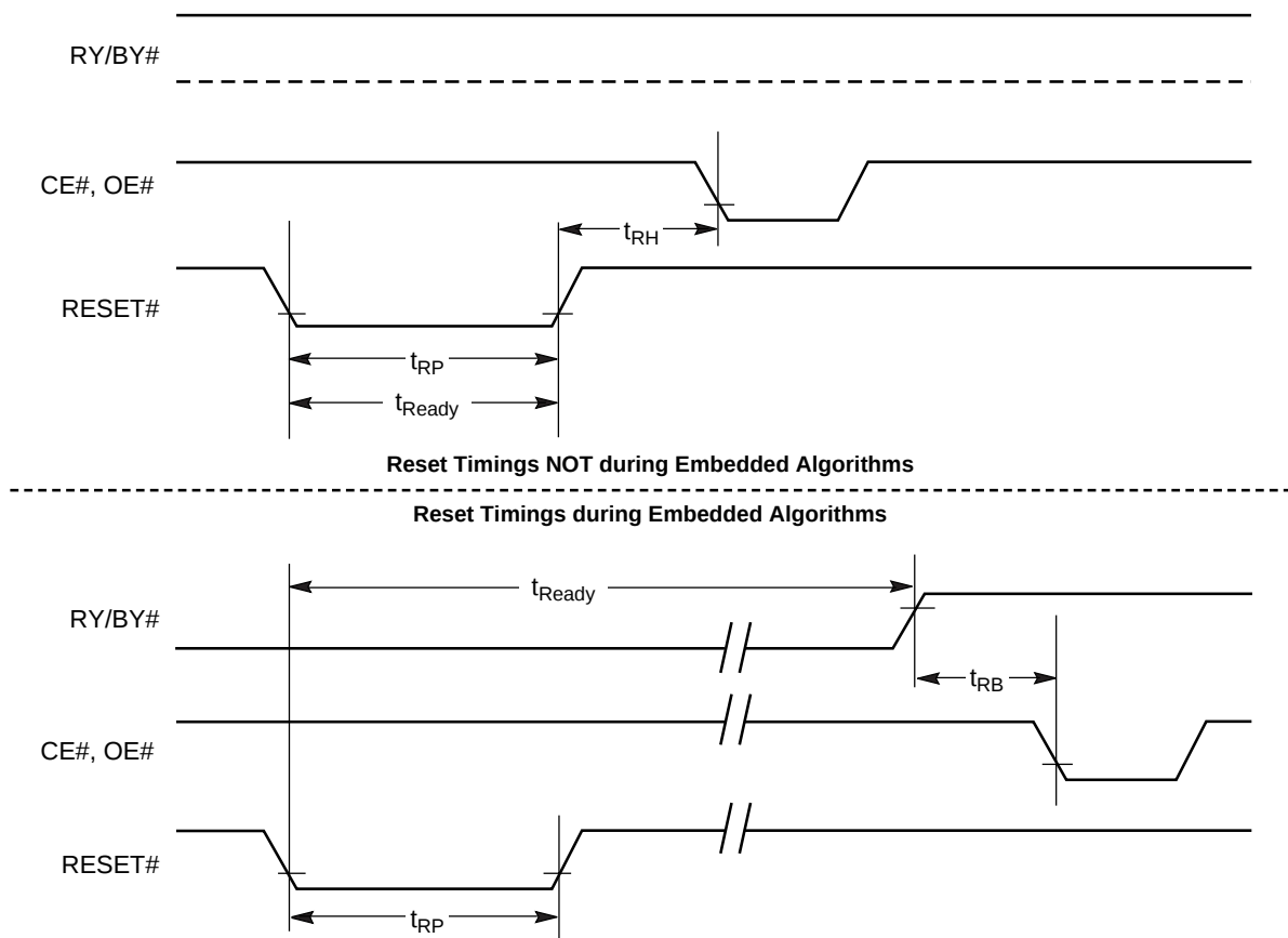
Figure 10. RESET# Timings
