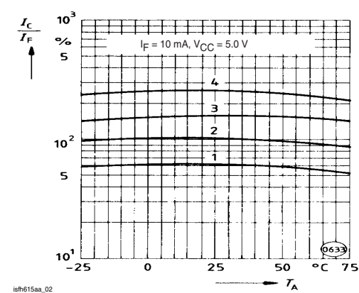
Fig. 2 Current Transfer Ratio (typical) vs. Temperature
