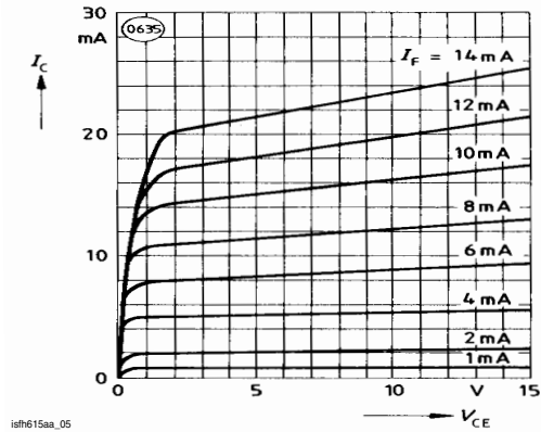
Fig. 5 Output Characteristics (typ.) Collector Current vs. Collector-Emitter Voltage
