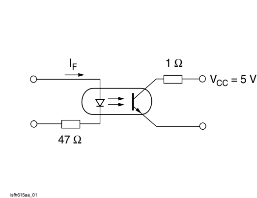
Fig. 1 Switching Operation (with Saturation)
