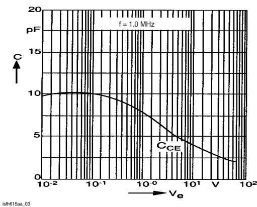
Fig. 3 Transistor Capacitance (typ.) vs. Collector-Emitter Voltage
