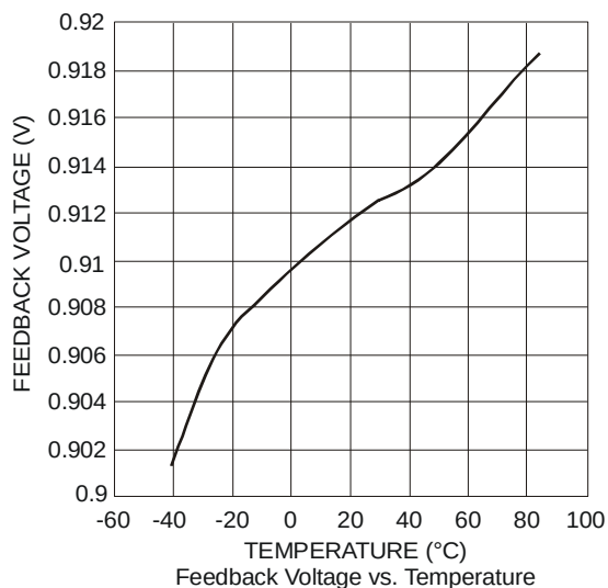
Feedback Voltage vs. Temperature
