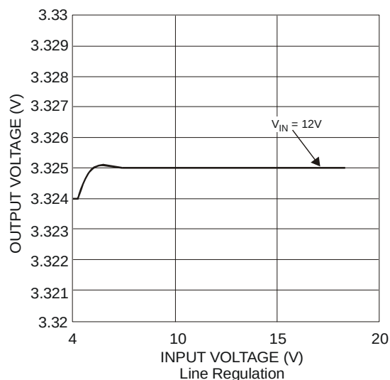
Line Regulation
