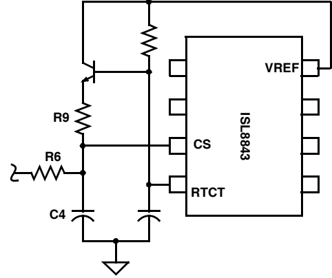
FIGURE 6. SLOPE COMPENSATION
