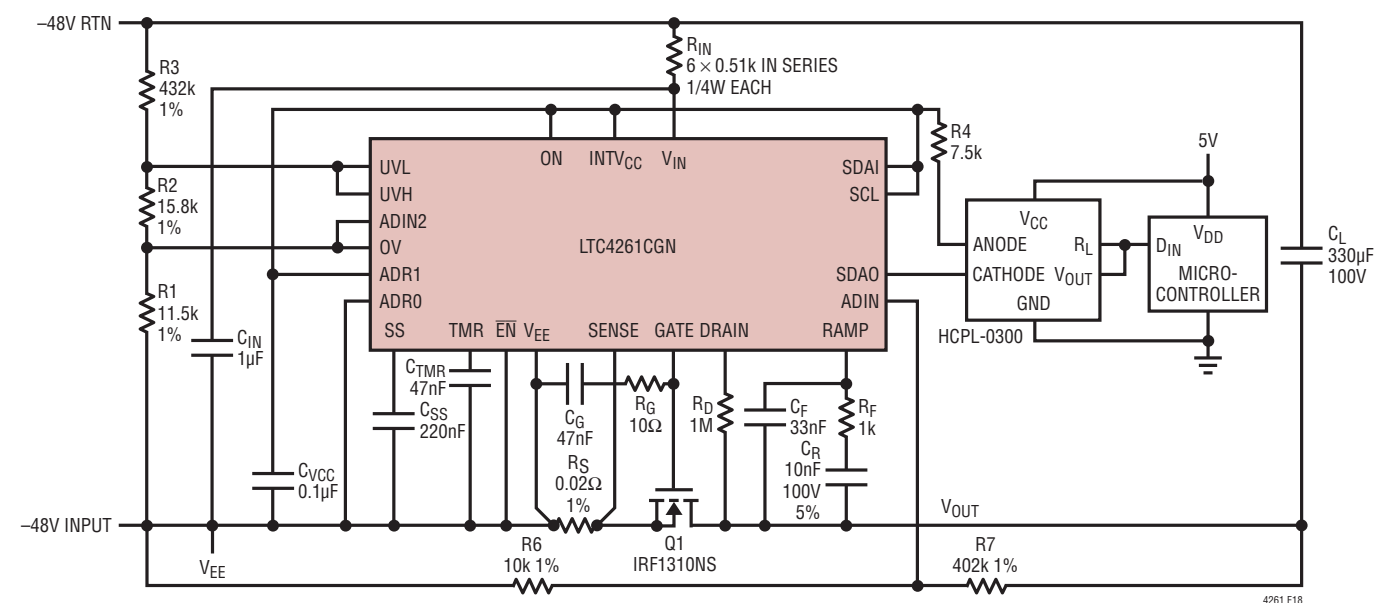
Figure 18. Application Circuit of the LTC4261 in Single-Wire Broadcast Mode
