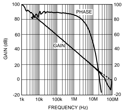
Figure 46. LMP7717 A_{VOL} vs. Frequency
