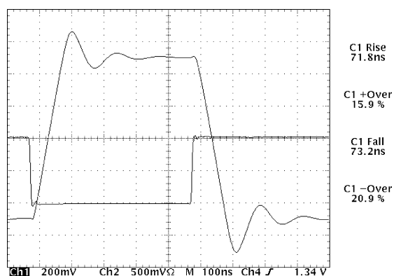
Figure 55. LMP7715 Response
