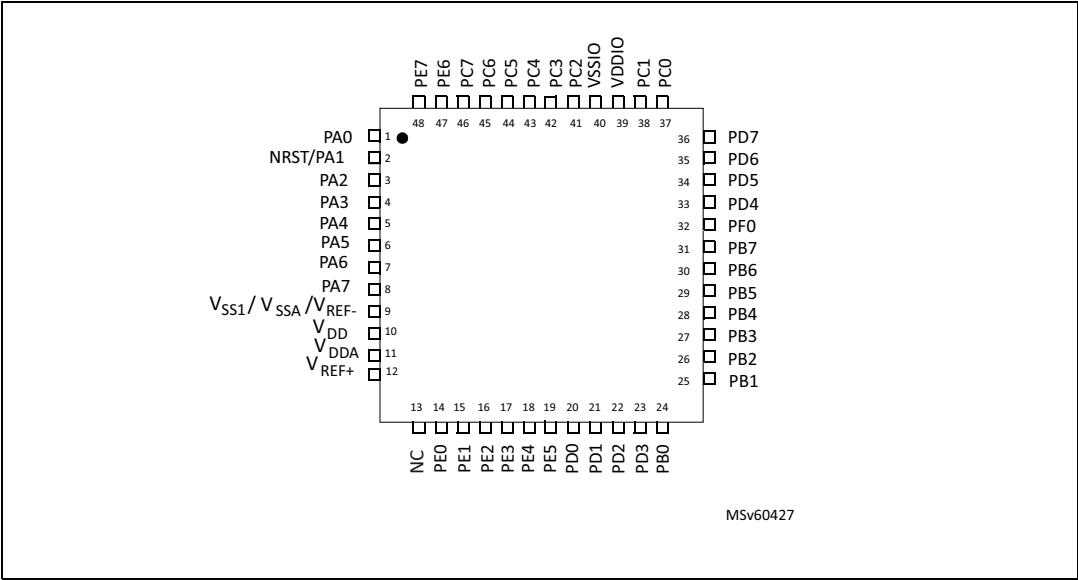
Figure 3. STM8L151Cx LQFP48 package pinout
