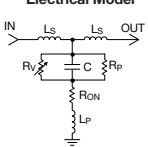
Electrical Model
