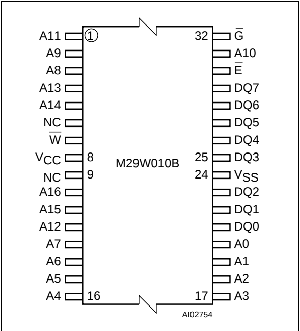
Figure 3. TSOP Connections
