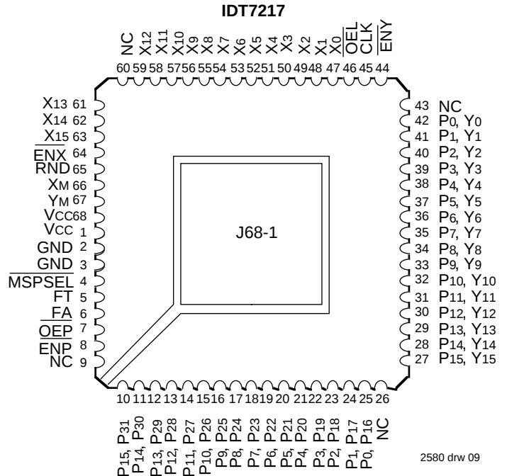
PLCC TOP VIEW
