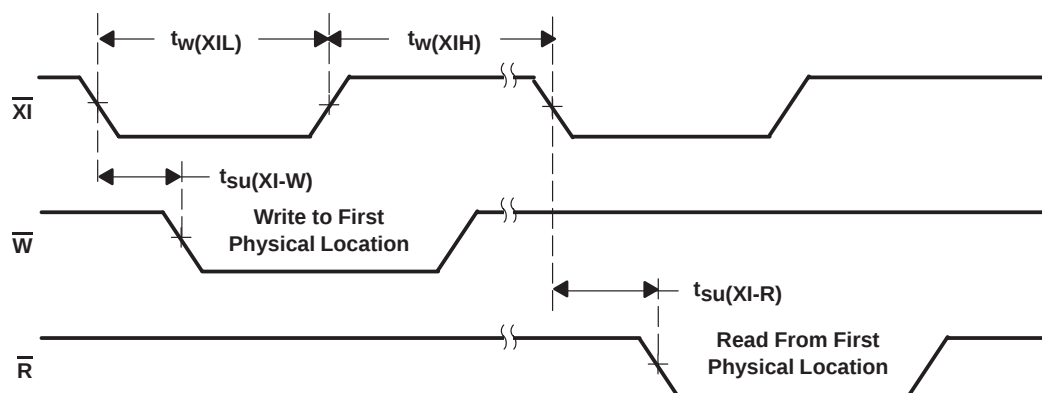
Figure 10. Expansion-In Waveforms
