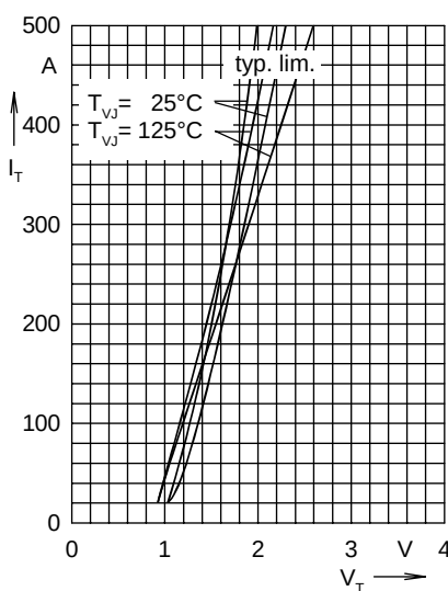
Fig. 2 On-state characteristics
