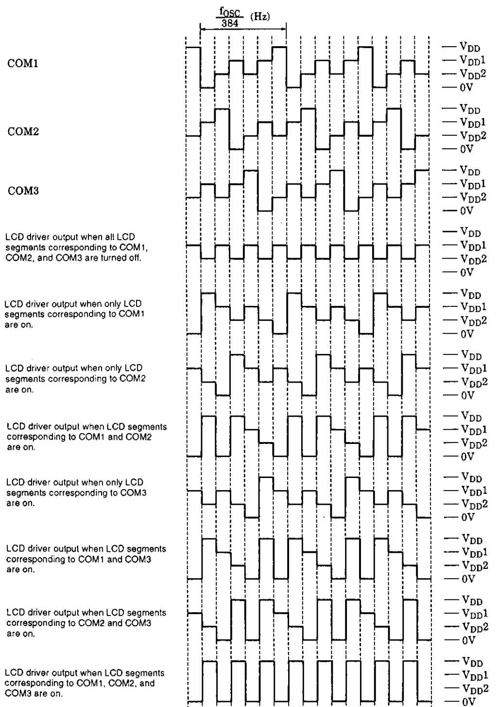
1/3-Duty - 1/3-Bias Waveforms
