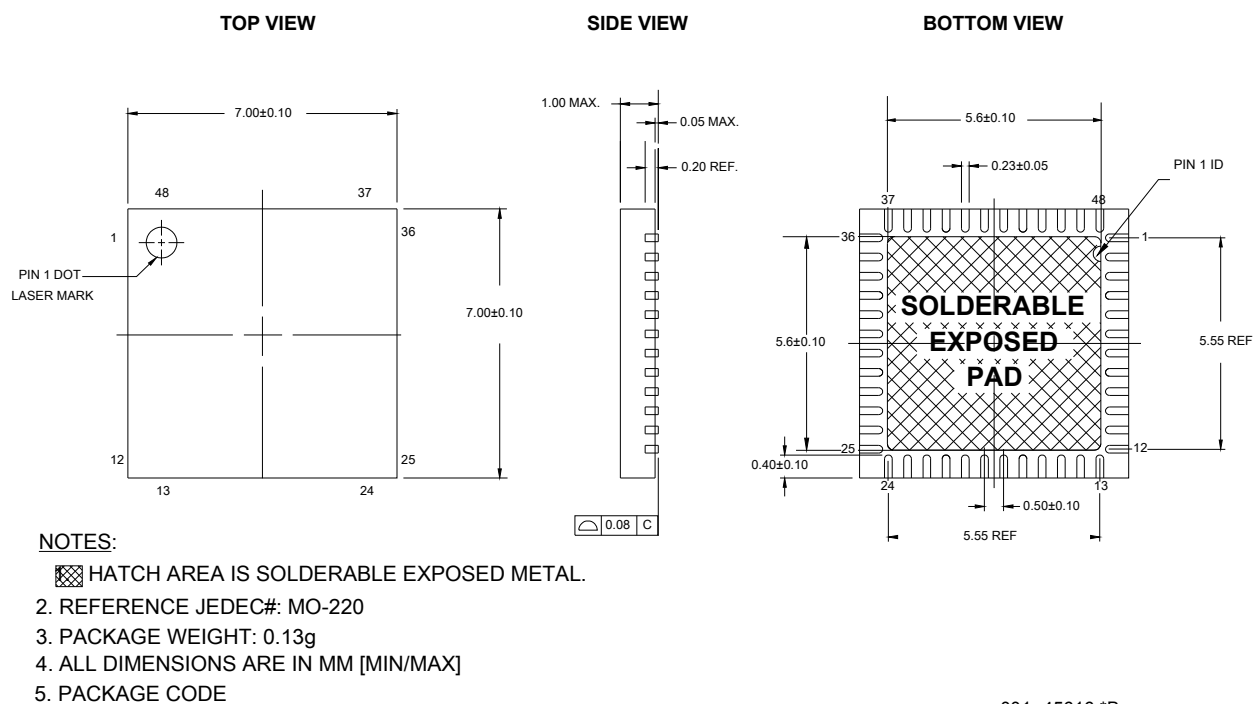
Figure 13-2. 48-pin QFN Package Outline
