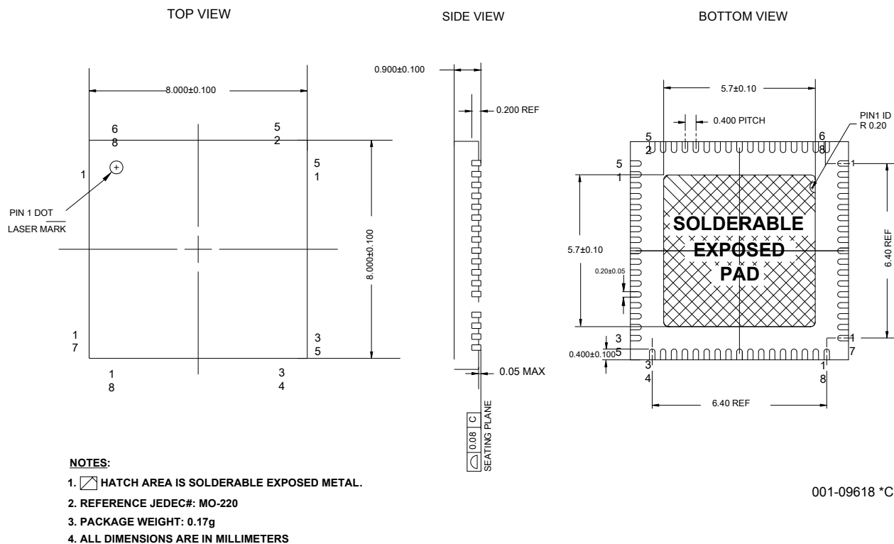
Figure 13-3. 68-pin QFN 8×8 with 0.4 mm Pitch Package Outline (Sawn Version)
