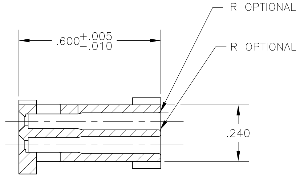
SECTION Y-Y
