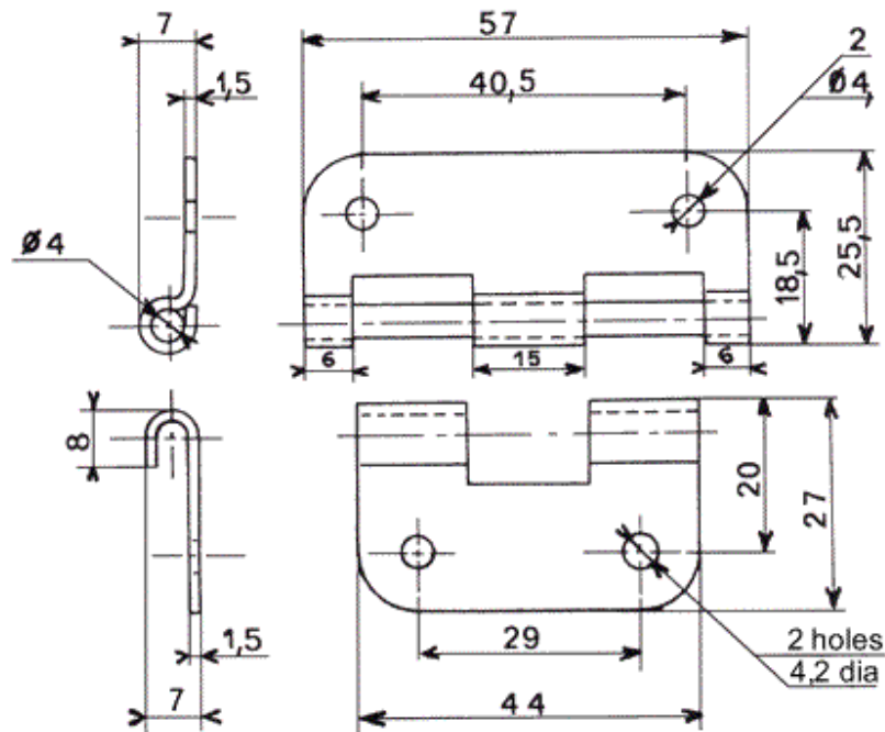
Type 421 - Horizontal Type
