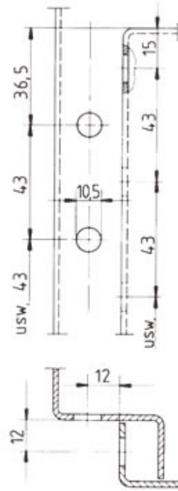
Panel preparation: hole size
