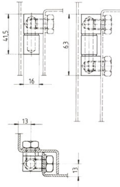
Mounting example
