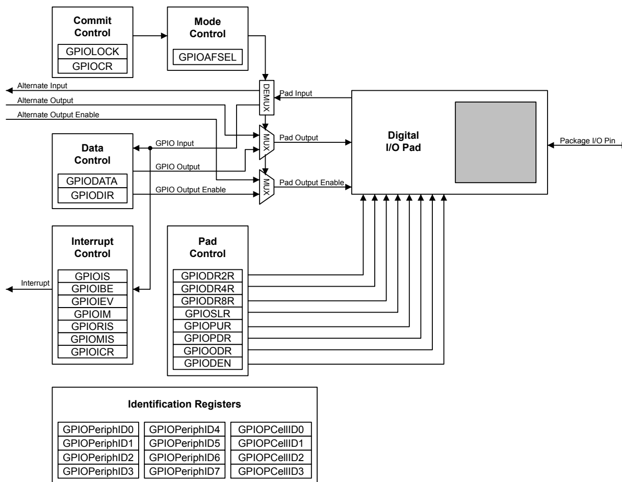
Figure 9-1. GPIO Port Block Diagram
