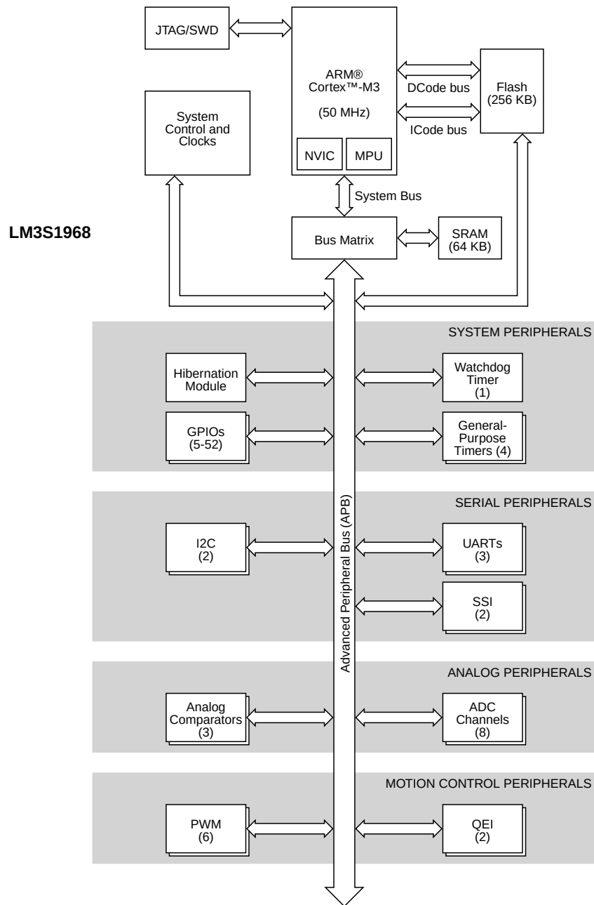
Figure 1-1. Stellaris® LM3S1968 Microcontroller High-Level Block Diagram
