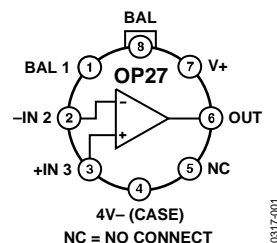
Figure 1. TO-99 (J-Suffix)
