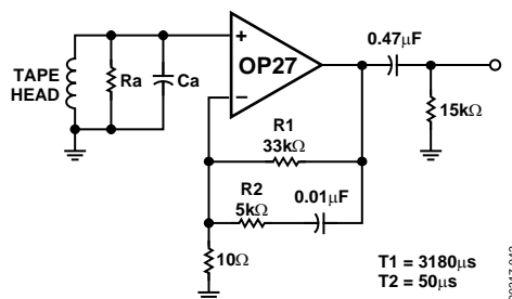
Figure 42. Tape-Head Preamplifier
