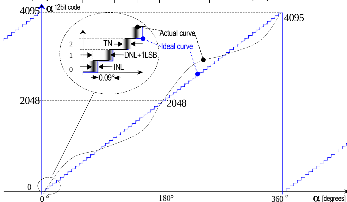
Figure 3: Integral and differential non-linearity (example)
