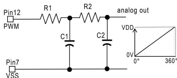
Figure 9: Simple 2 nd order passive RC lowpass filter
