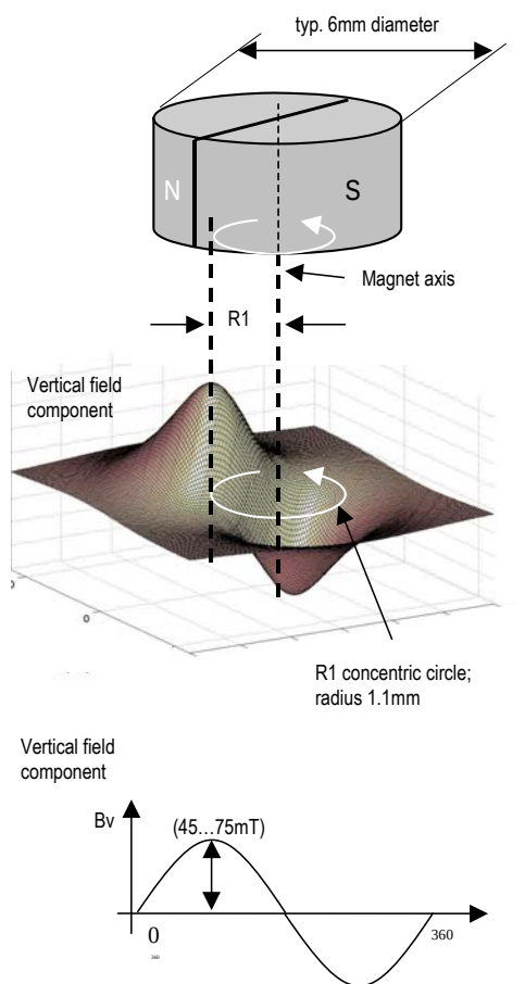
Figure 17: Typical magnet (6x3mm) and magnetic field distribution
