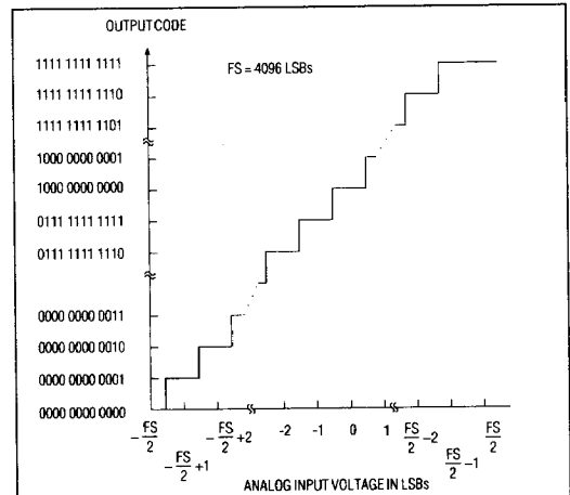
Figure 14. Ideal Bipolar Transfer Function
