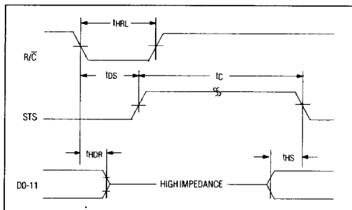
Figure 6. Low Pulse for R/C in Stand-Alone Mode
