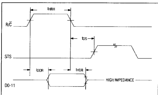
Figure 7. High Pulse for R/C in Stand-Alone Mode
