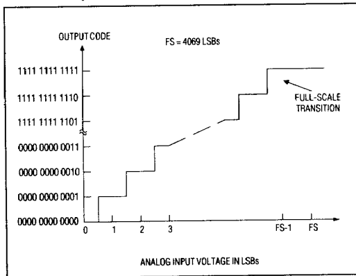
Figure 12. Ideal Unipolar Transfer Function
