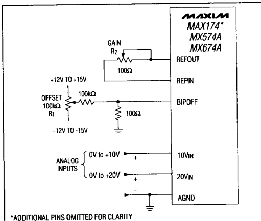
Figure 13. Unipolar Input Connections
