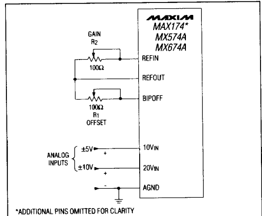
Figure 15. Bipolar Input Connections
