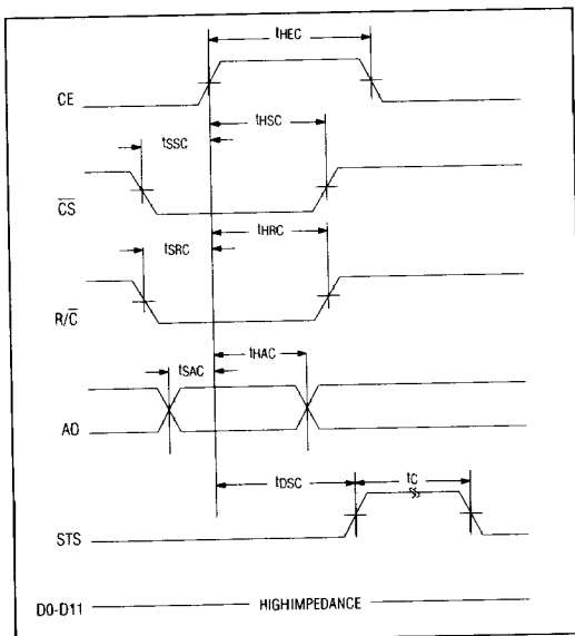
Figure 4. Convert Start Timing
