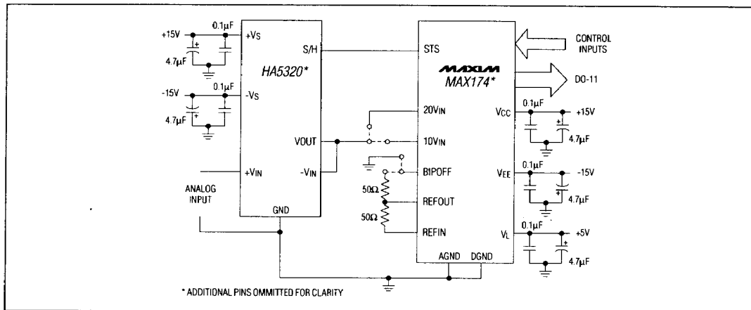
Figure 11. MAX174 to HA5320 Sample-and-Hold Interface
