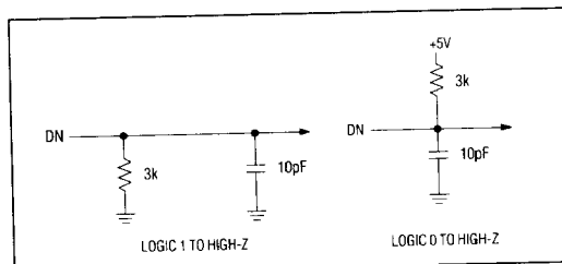
Figure 2. Load Circuit for Output Float Delay Test
