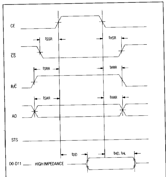
Figure 5. Read Timing
