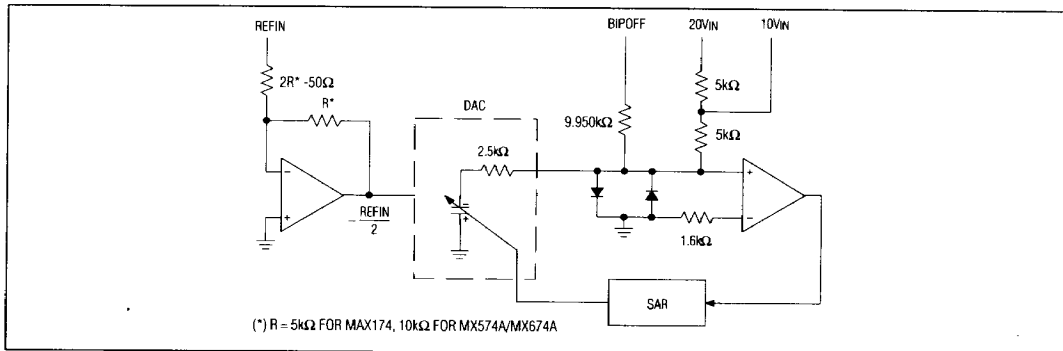
Figure 3. Analog Equivalent Circuit
