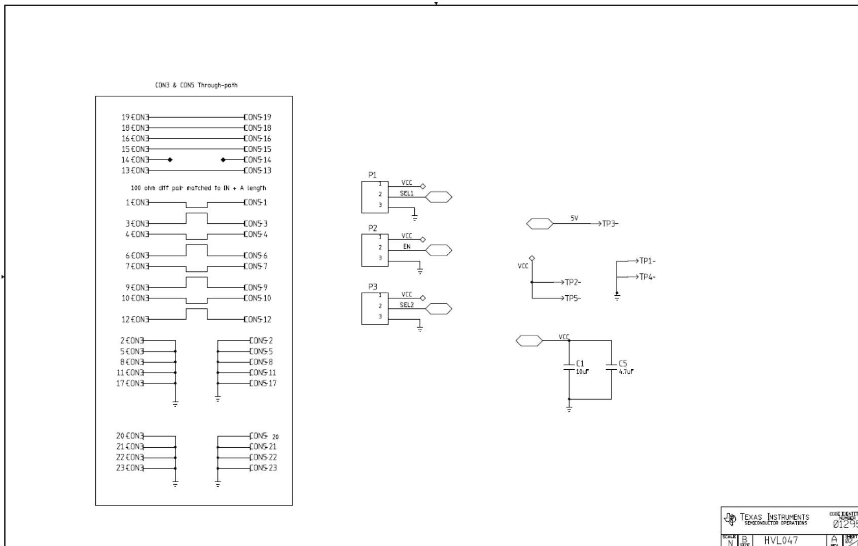
Figure 5. Schematic (2 of 2)
