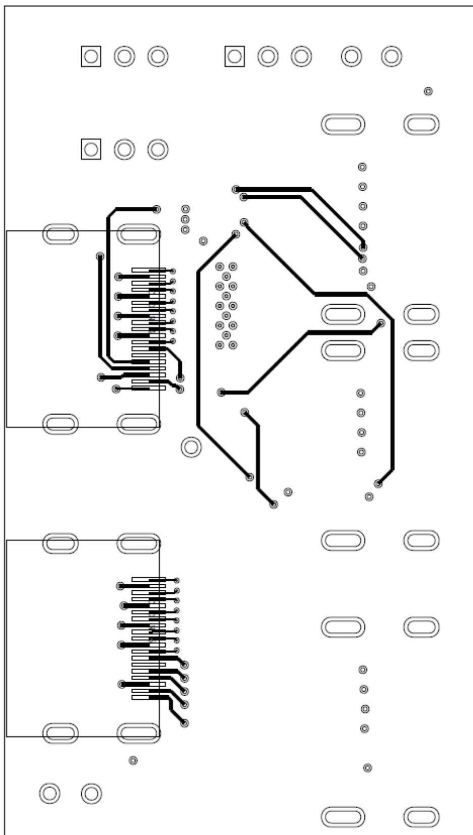
Figure 9. Bottom Layer
