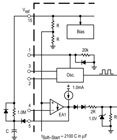
Figure 20. Soft-Start Circuit
