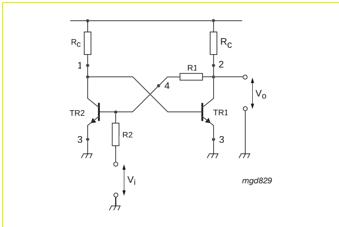
Schmitt trigger
