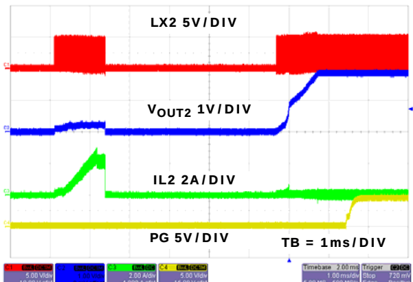
FIGURE 43. OUTPUT SHORT CIRCUIT RECOVERY CHANNEL 2
