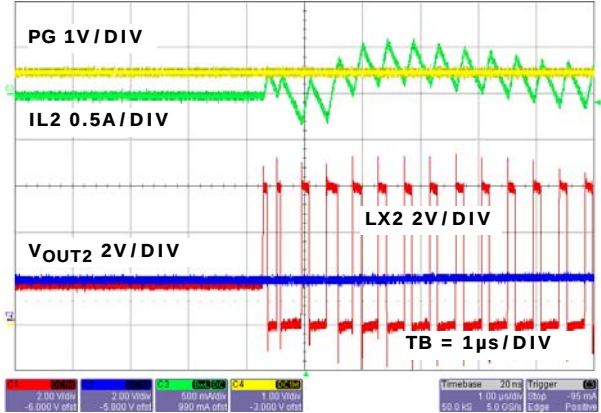
FIGURE 39. RECOVERY FROM HARD SHORT NEGATIVE CURRENT WAVEFORMS V_{OUT2} CHANNEL 2
