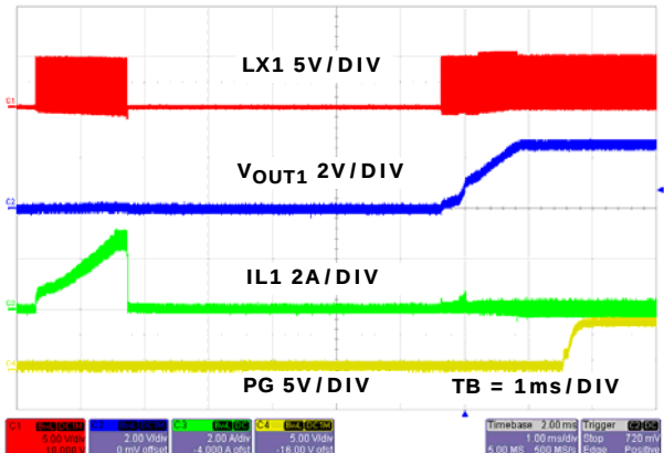
FIGURE 41. OUTPUT SHORT CIRCUIT RECOVERY CHANNEL 1
