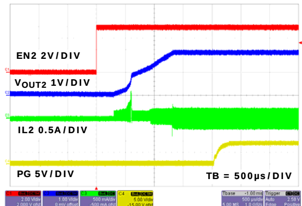
FIGURE 25. SOFT-START WITH NO LOAD CHANNEL 2 (PWM)
