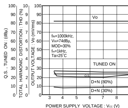
Fig.8 AM characteristics vs. power supply voltage
