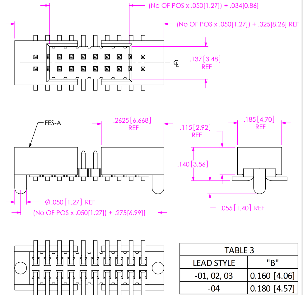
FIG 4 -DV-SA OPTION (SEE NOTES 6 & 7) FTS-106-02-XX-DV-SA SHOWN (DIFFERENT AS SHOWN, OTHERWISE SAME AS FIG 1) NOTE: 4 POSITIONS MUST BE ADDED TO PART CALLOUT TO ACHIEVE DIMS
