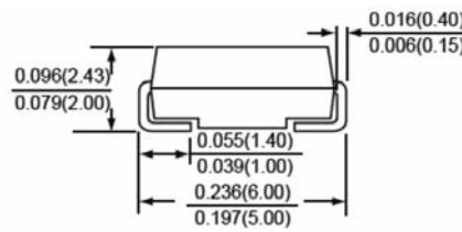
SMB/DO-214AA
