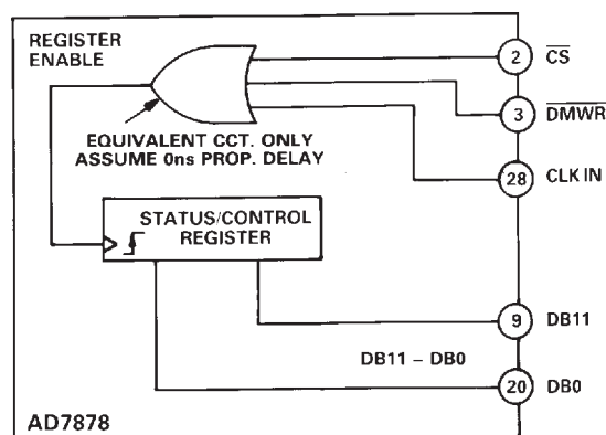
Figure 7. \overline{\text{DMWR}} Internal Logic
