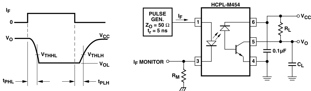
Figure 6. Switching Test Circuit.
