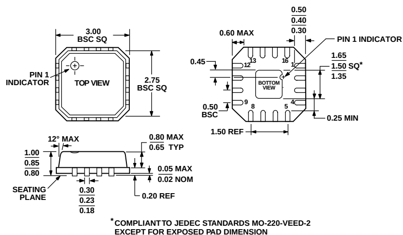
Figure 27. 16-Lead Lead Frame Chip Scale Package [LFCSP] (CP-16)
