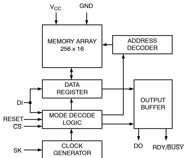
Figure 1. Block Diagram
