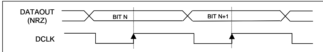
Figure 11: DATAOUT timing
