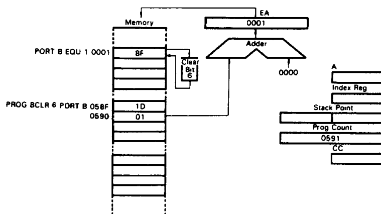
Figure 36 Example of Bit Set/Clear Addressing
