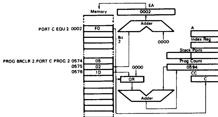
Figure 37 Example of Bit Test and Branch Addressing
