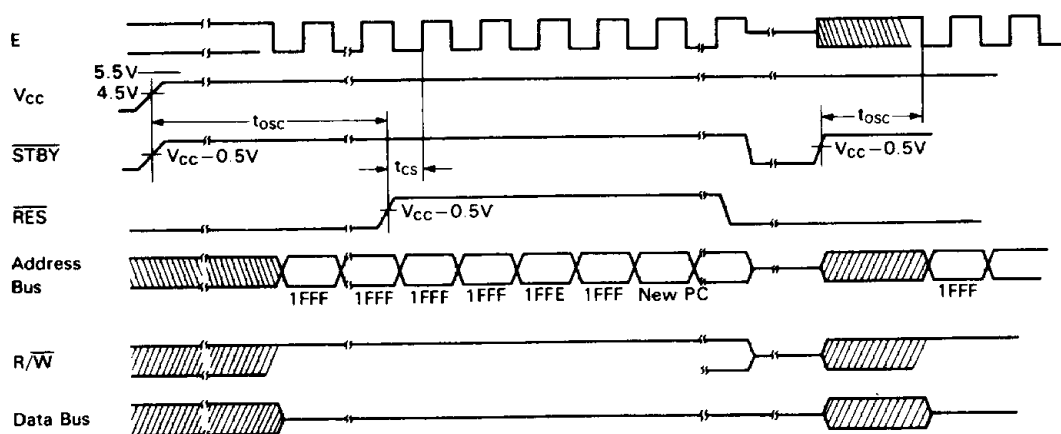
Figure 5 Reset Timing
