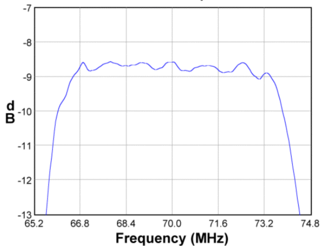
Passband Response
