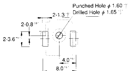
PC Board Layout Acceptable Board Thickness : 1.6
