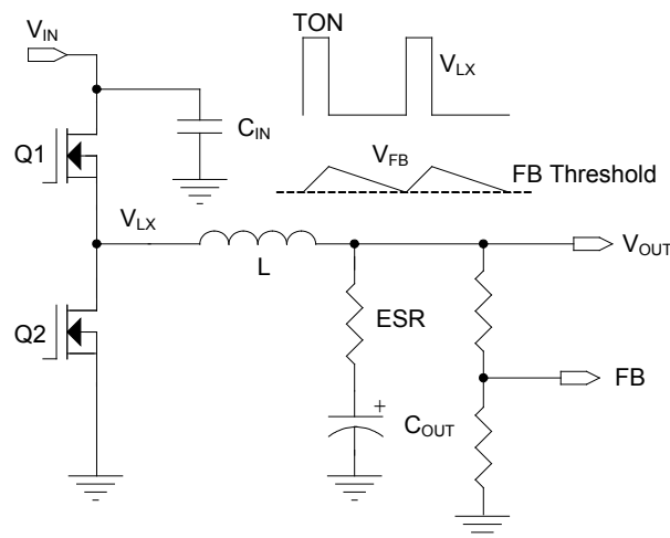
Figure 1 — PWM Control Method, V_{OUT} Ripple
