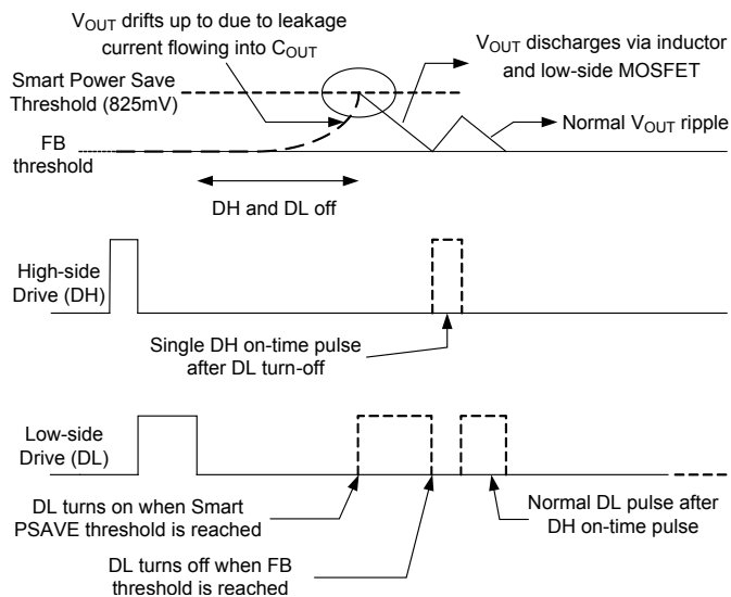
Figure 6 — Smart PSAVE
