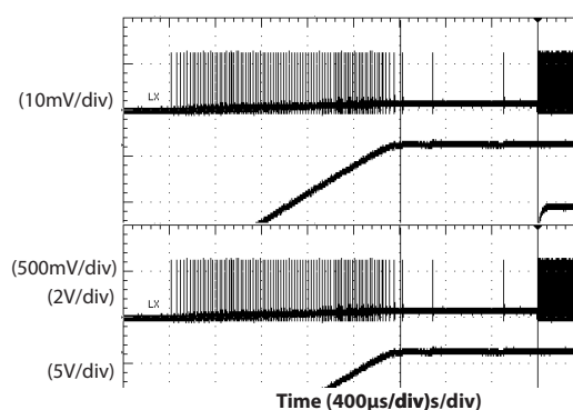
Figure 8 — Soft-start Timing Diagram
