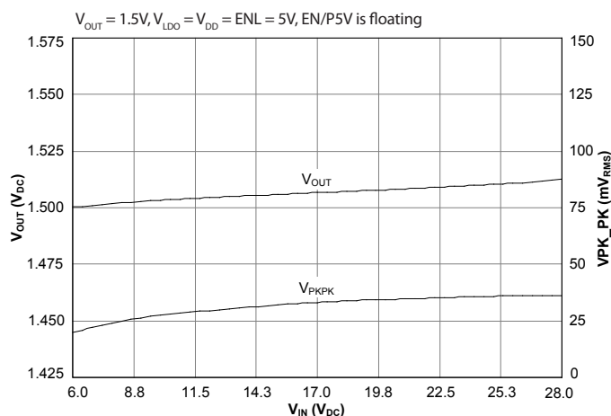
V_{OUT} vs. Line — Forced Continuous Mode
