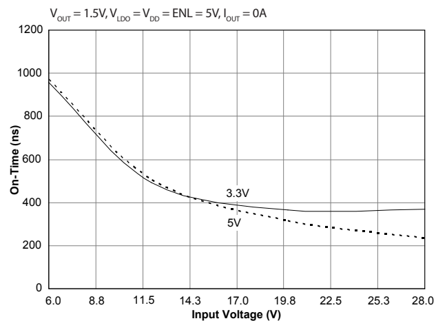
On Time vs. Line
