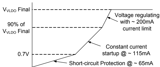
Figure 11 — LDO Start-Up
