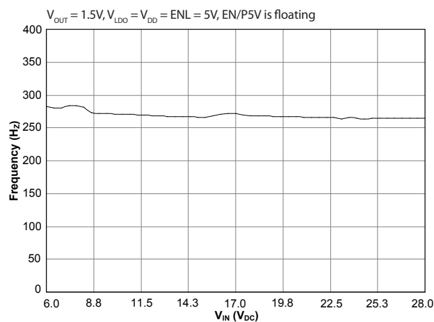
Frequency vs. Line — FCM Mode
