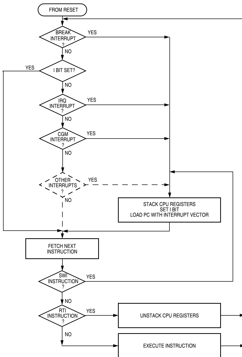
Figure 15-10. Interrupt Processing
